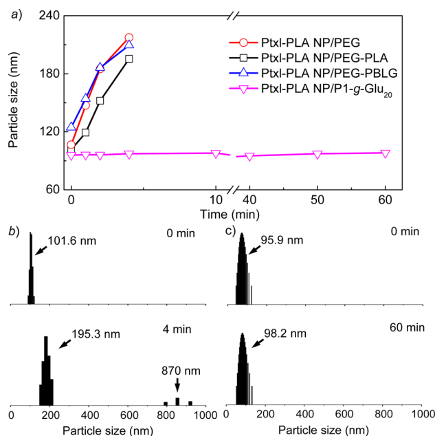
Figure 2. (a) Stability of Ptxl-LA NPs in PBS (1 \times ) after coated with mPEG5k (PEG), mPEG5k-PLA (PEG-PLA), PEG-PBLG, or P1- g -Glu 20 ; (b) DLS spectra of Ptxl-LA/PEG-PLA NP in PBS buffer after 0 and 4 min; (c) DLS spectra of Ptxl-LA/P1- g -Glu 20 NP in PBS buffer after 0 and 60 min.
